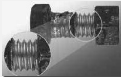
Engagement area of rusty bolt that DID have LOCTITE® threadlocker applied.
