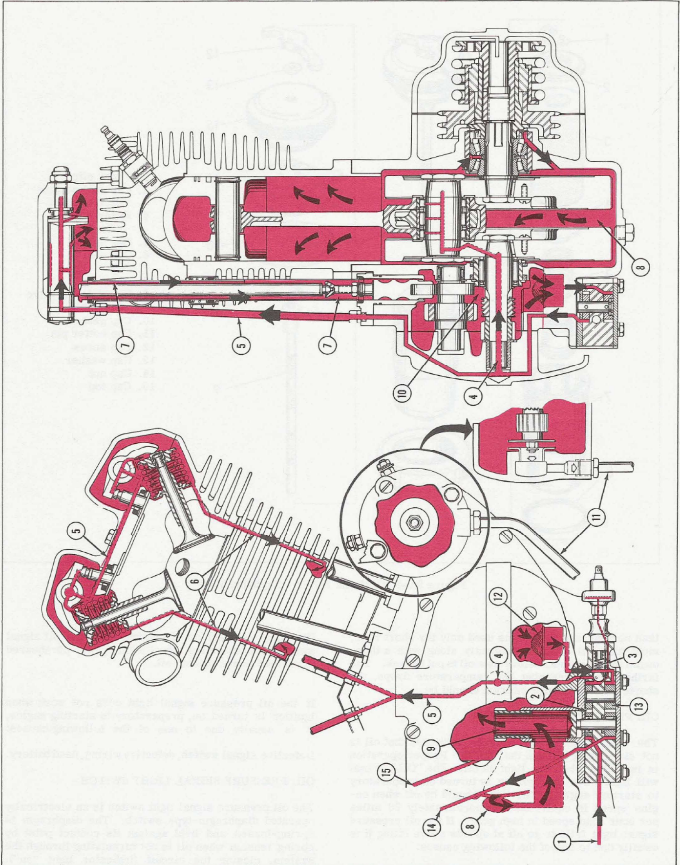
Figure 3A-6. Oiling System
